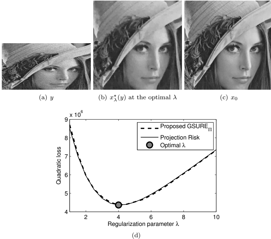
Figure 1: Illustration of the selection of \lambda by minimizing \text{GSURE}_{\Pi} in a super-resolution problem ( Q/N = 0.5 ) with anisotropic total variation regularization. (a) The observed image y . (b) A solution x_\lambda^*(y) of (\mathcal{P}_\lambda(y)) at the optimal \lambda (the one minimizing \text{GSURE}_{\Pi} ). (c) The underlying true image x_0 . (d) Projection risk \text{Risk}_{\Pi} and its \text{GSURE}_{\Pi} estimate obtained from (10) using k = 1 random realization.
