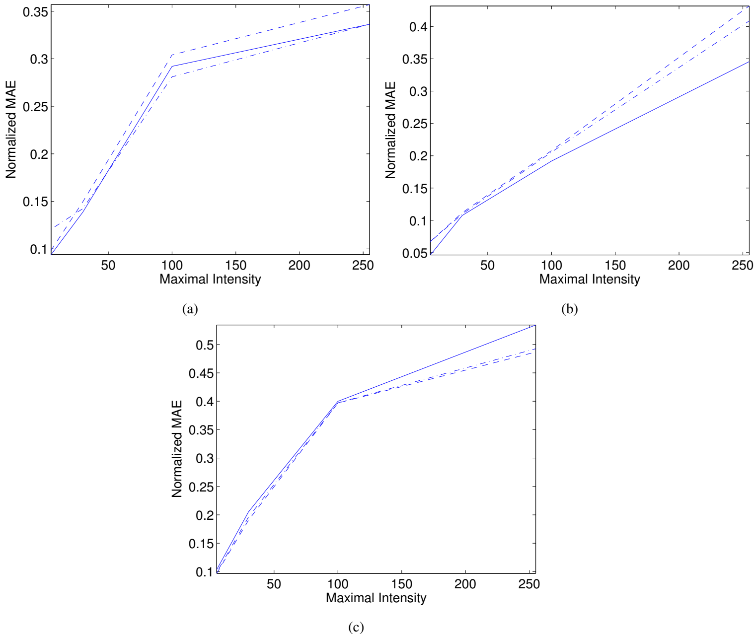
Figure 8. Impact of the dictionary on deconvolution performance as a function of the maximal intensity level for several test images: (a) Neuron phantom, (b) Cell and (c) LinesGaussians images. Solid line indicates the TI-DWT, dashed line corresponds to the curvelet transform, and dashed-dotted line to the dictionary built by merging both wavelets and curvelets.
