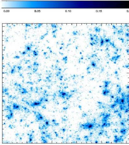
Figure 1. Simulated weak lensing convergence map for the \Lambda CDM cosmological model with \Omega_m = 0.3 and \Omega_\Lambda = 0.7 . The region shown is 1^\circ \times 1^\circ .
